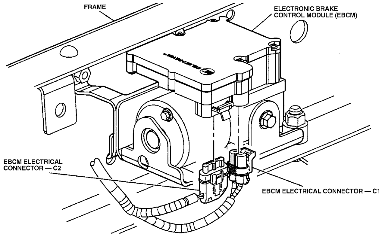
Figure G2019-4 Kelsey-Hayes EBC 325 & EBC 325S (w/NW7) used on Avalanche, Silverado, S10, Trailblazer, Tahoe, Astro and Safari
