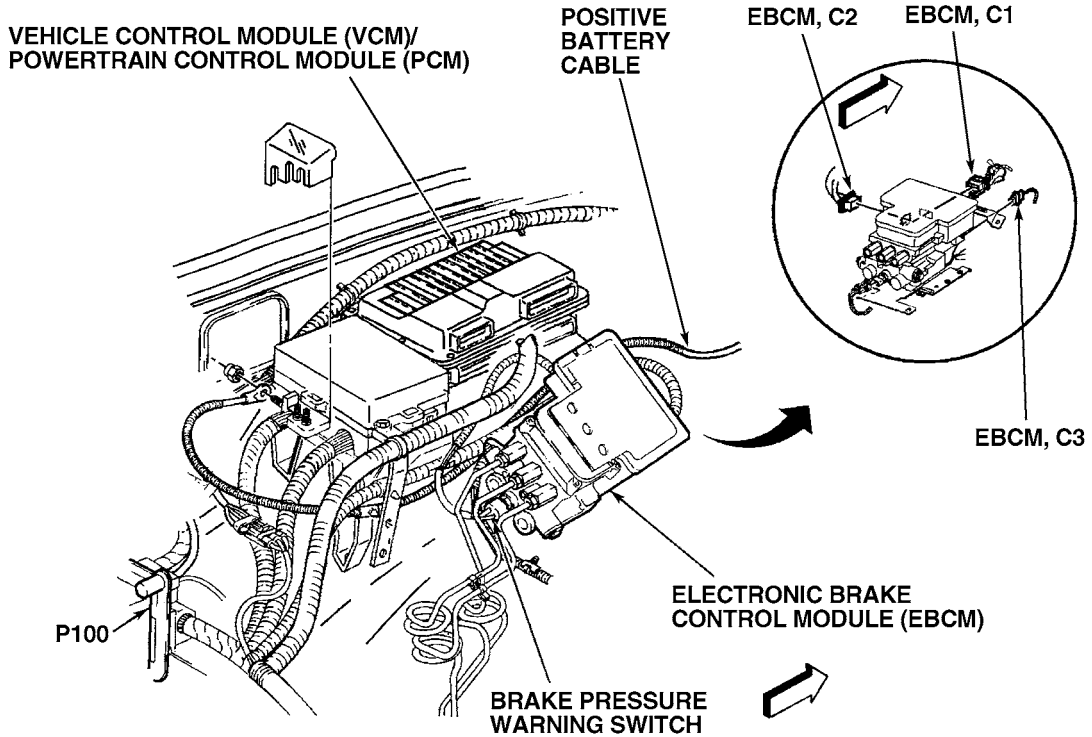
Figure G2019-9 Kelsey-Hayes EHCU used on C- & K-Series pickups
