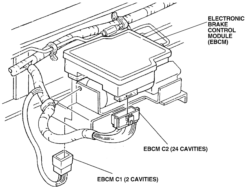
Figure G2019-10 Kelsey-Hayes ABS for a P-Chassis (Workhorse)
