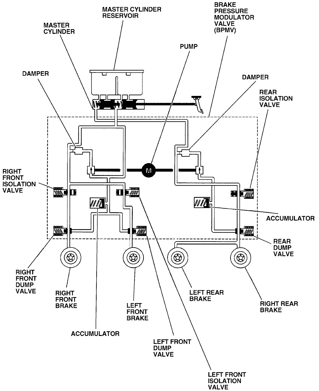
Figure G2019-7 Kelsey-Hayes EBC 325 BPMV hydraulic flow
