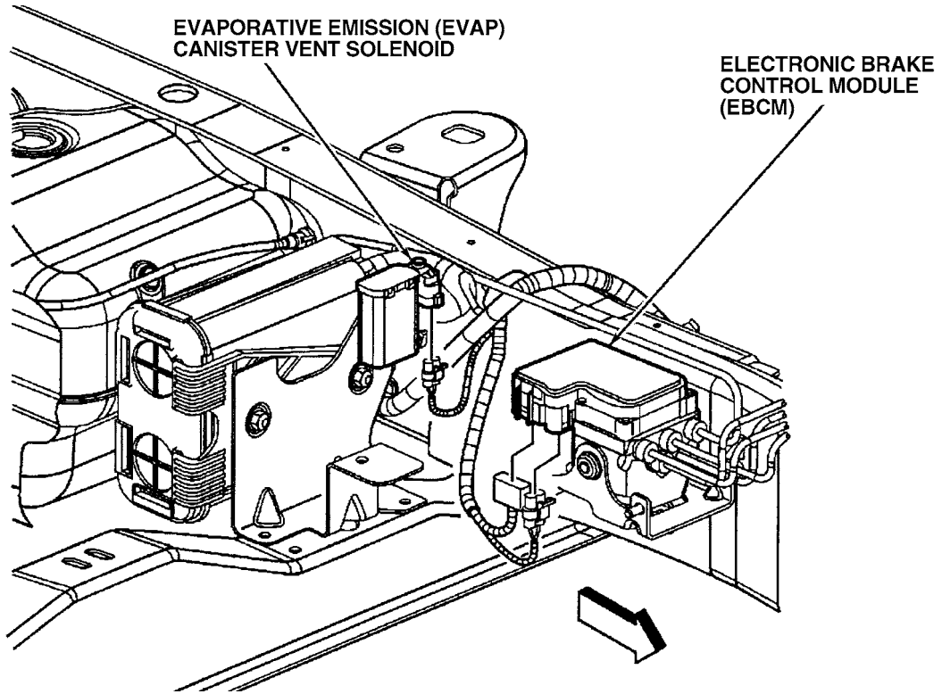
Figure G2019-8 Kelsey-Hayes 325 EV used on a G-Series van
