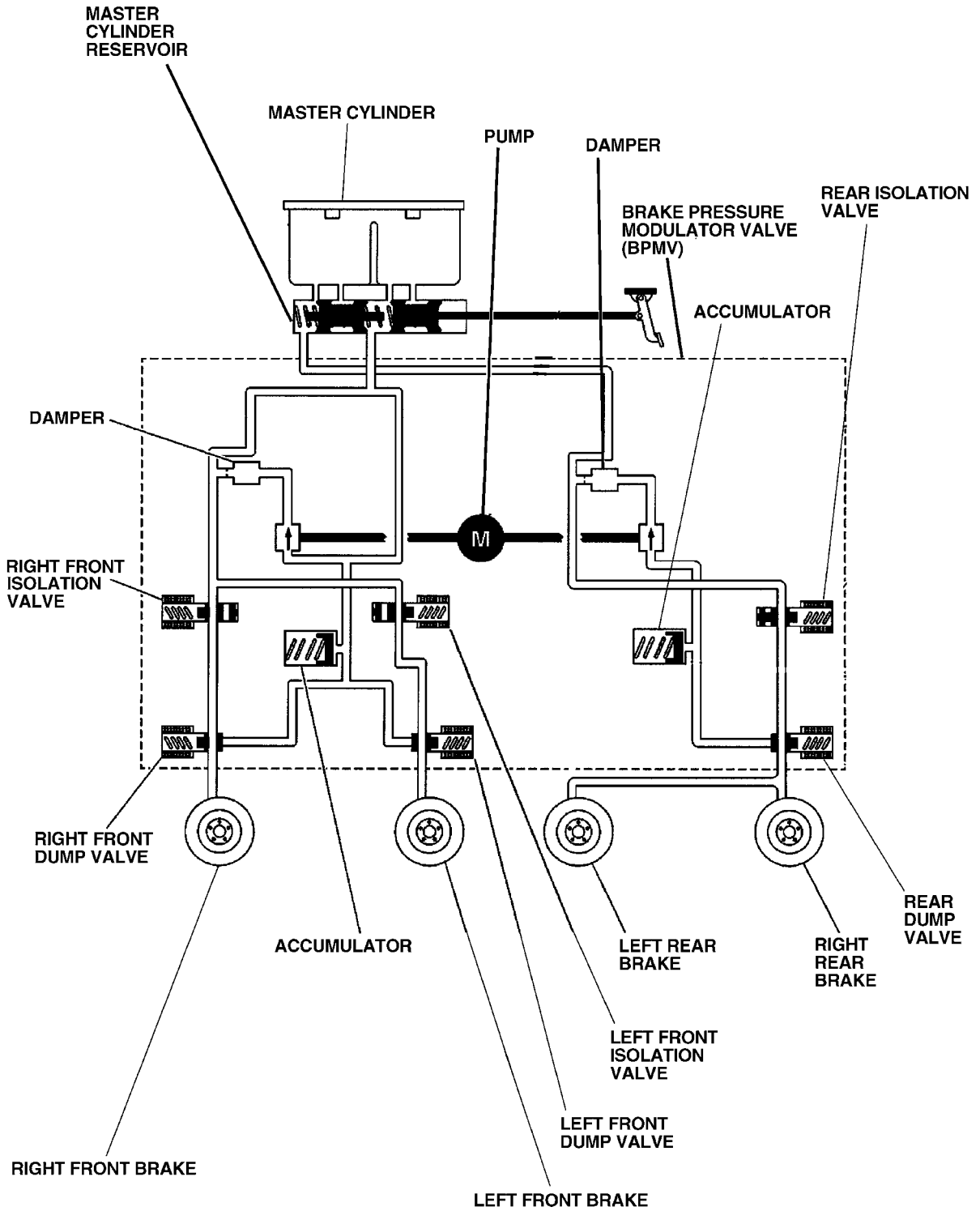
Figure G2019-5 Kelsey-Hayes EBC 325 & EBC 325S (w/NW7) BPMV hydraulic flow
