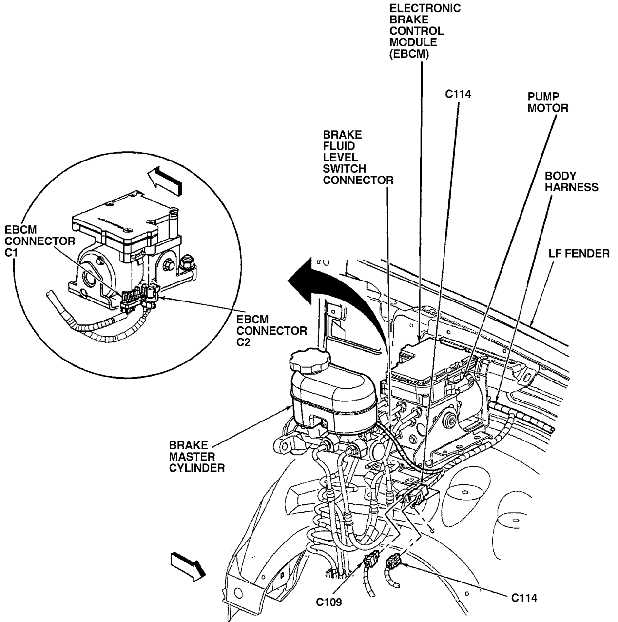
Figure G2019-6 Kelsey-Hayes EBC 325 used on 2000 and later S10 Blazer and Pickup
