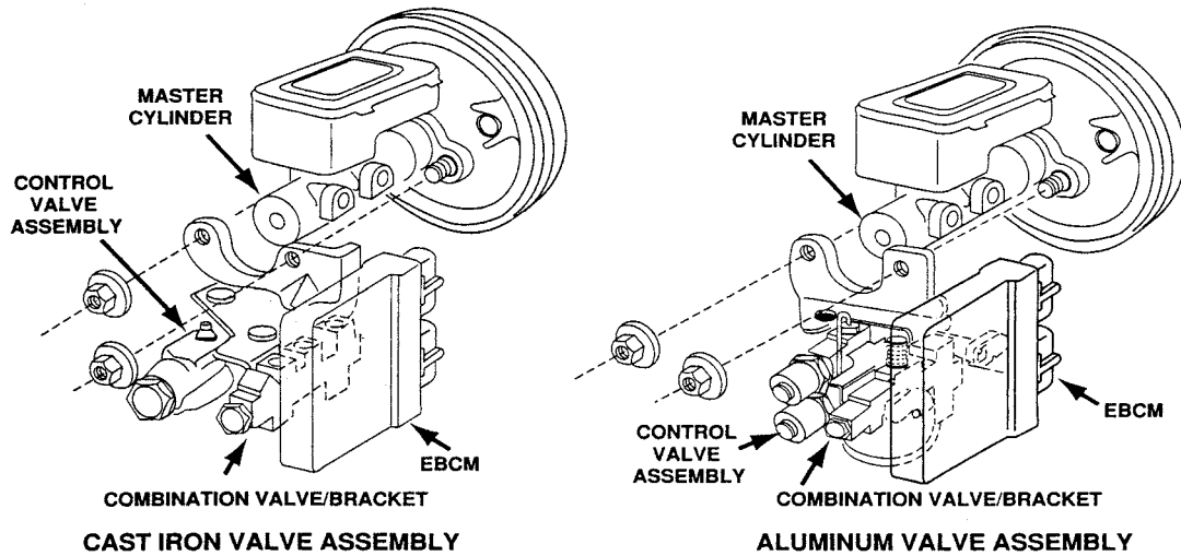
Figure G2019-3 RWAL control valve assemblies
