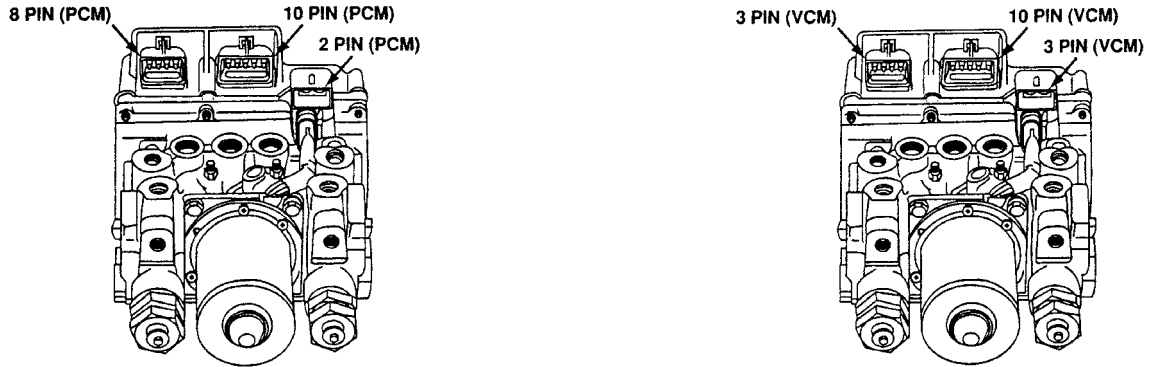
Figure G2019-2 Kelsey-Hayes EBC4 4WAL system connector pin configuration
