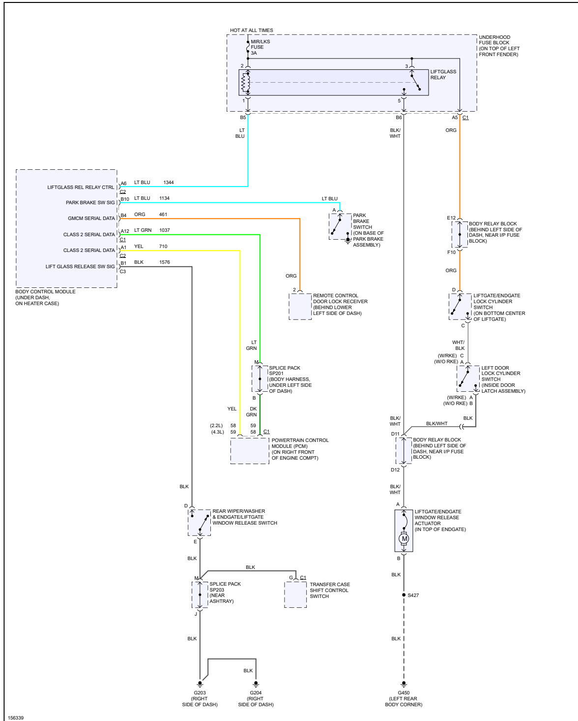
Fig 1: Liftgate/Endgate Release Circuit
