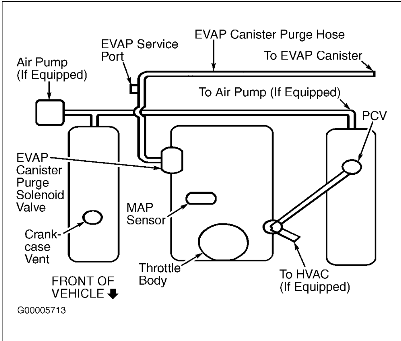
Fig 6: Vacuum Diagram - 4.3L SFI (VIN W) "C", "G", "K", "L", "M", "S" & "T" Series
