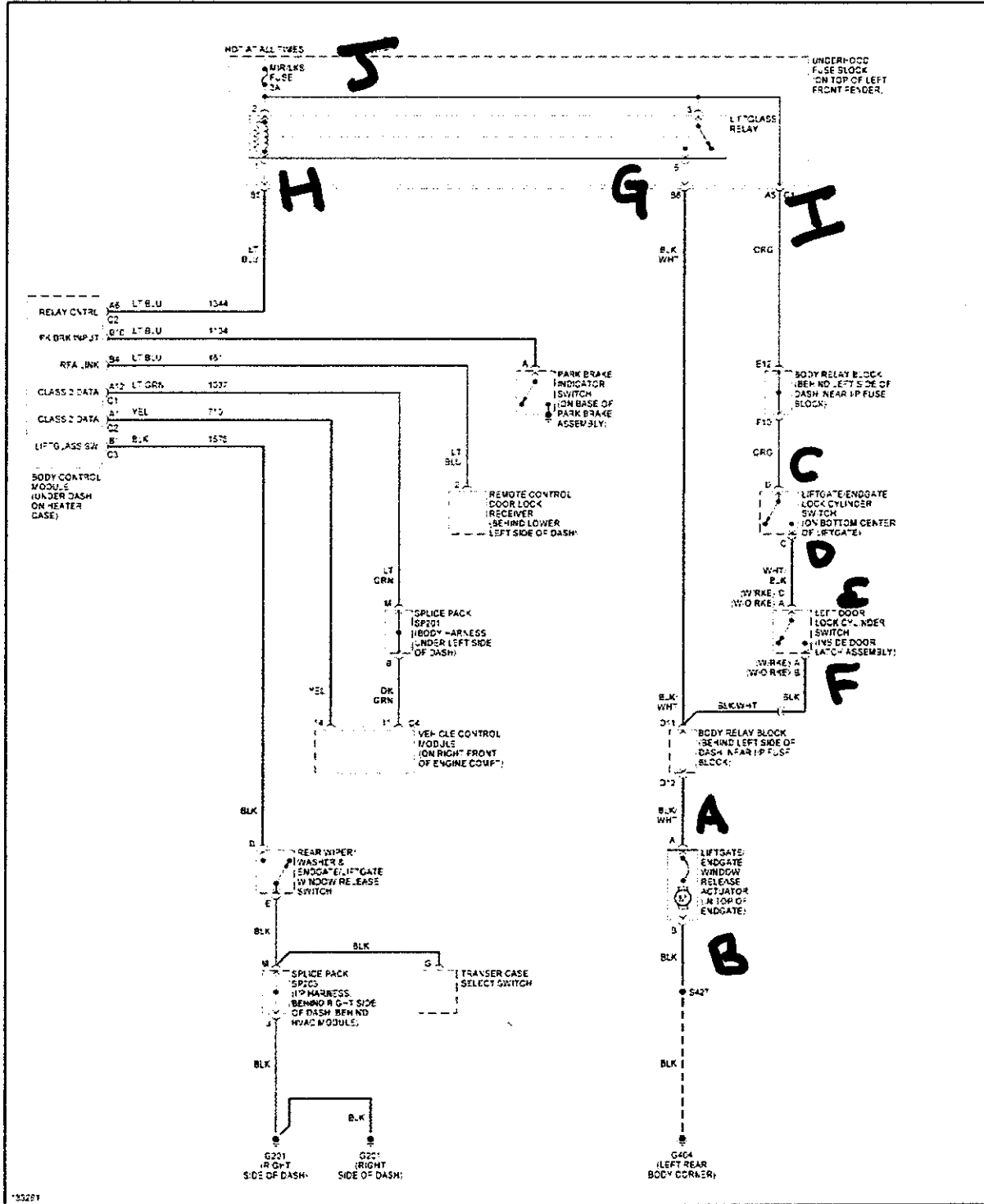
Fig. 57: Liftgate/Endgate Release Circuit
