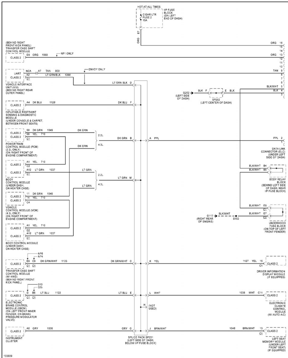
Fig. 10: Computer Data Lines
