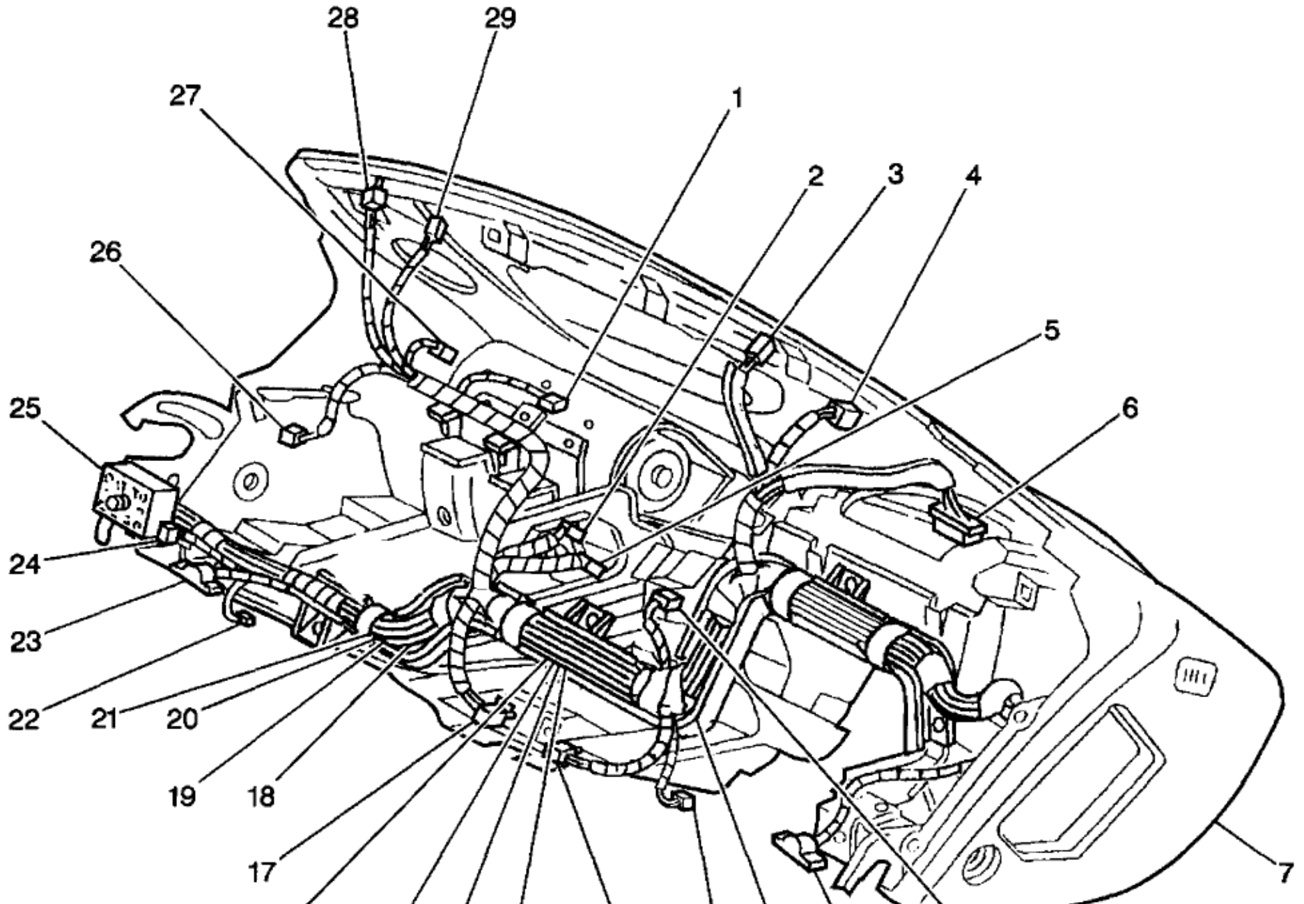
IP Wiring Harness Composite View (With Auto A/C)
