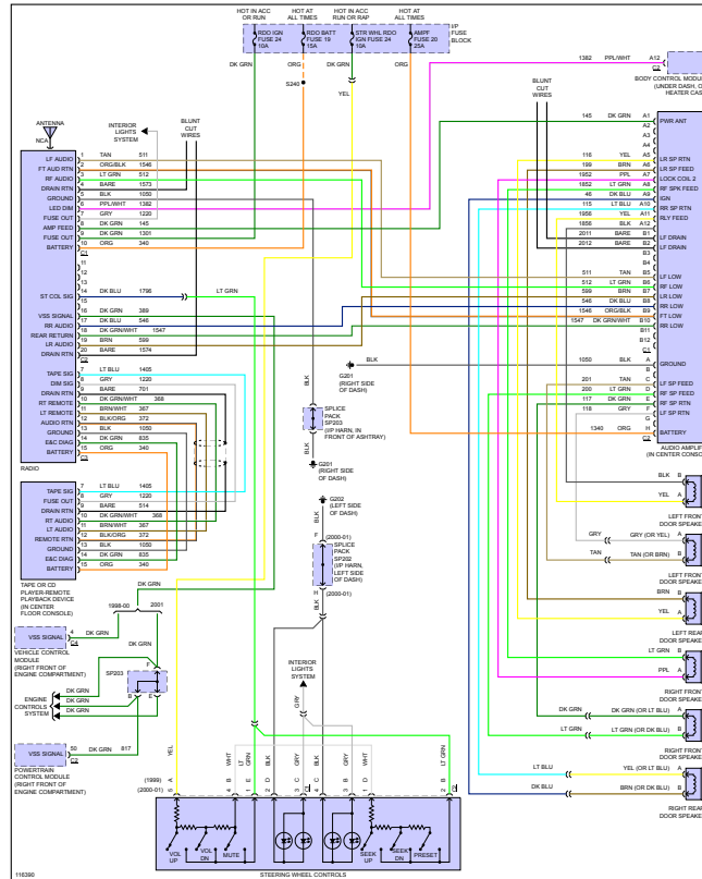
Fig 1: Radio Circuit, W/ Amplifier
