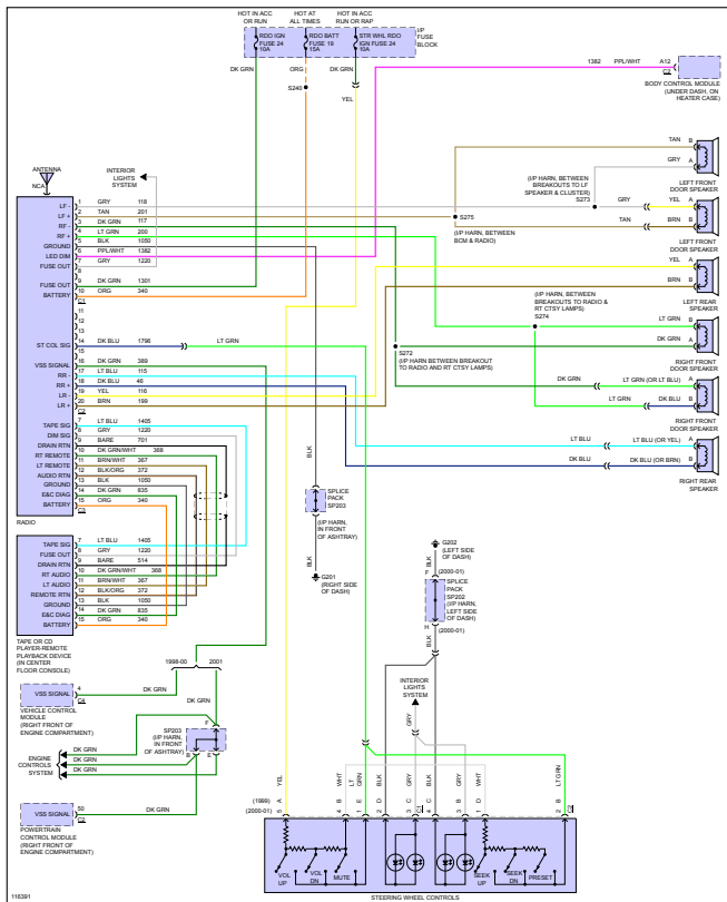
Fig 2: Radio Circuit, W/O Amplifier
