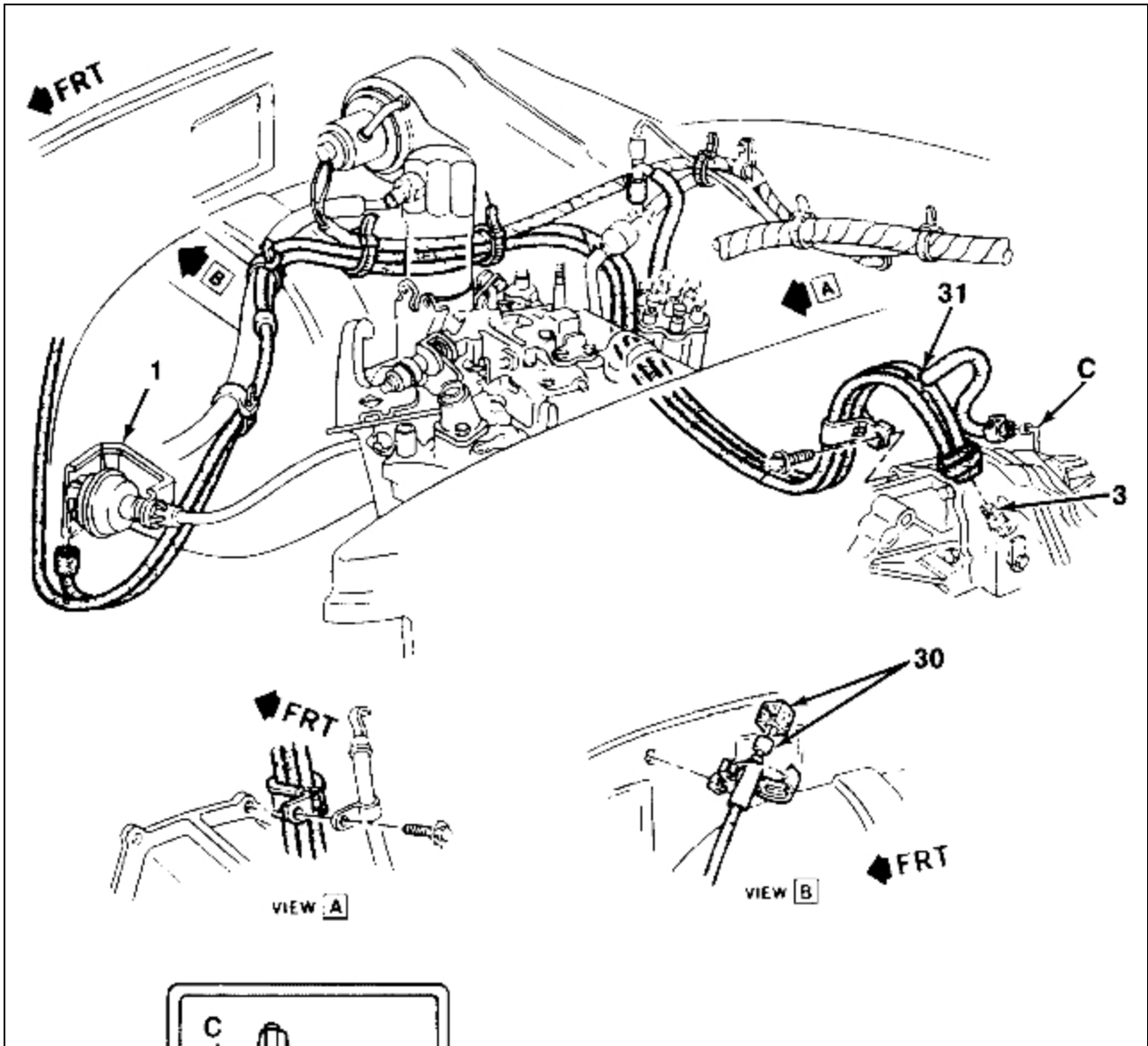
Fig 5: Vacuum Line Routing and Schematic
