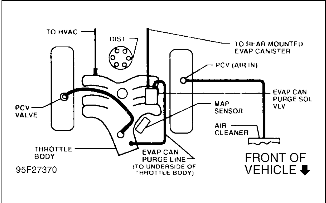
Fig 1: 4.3L CPI "S" & "T" Series Calif./Fed. All Transmissions (YBD, YBP, YBR, YBS, YBT & YJL)
