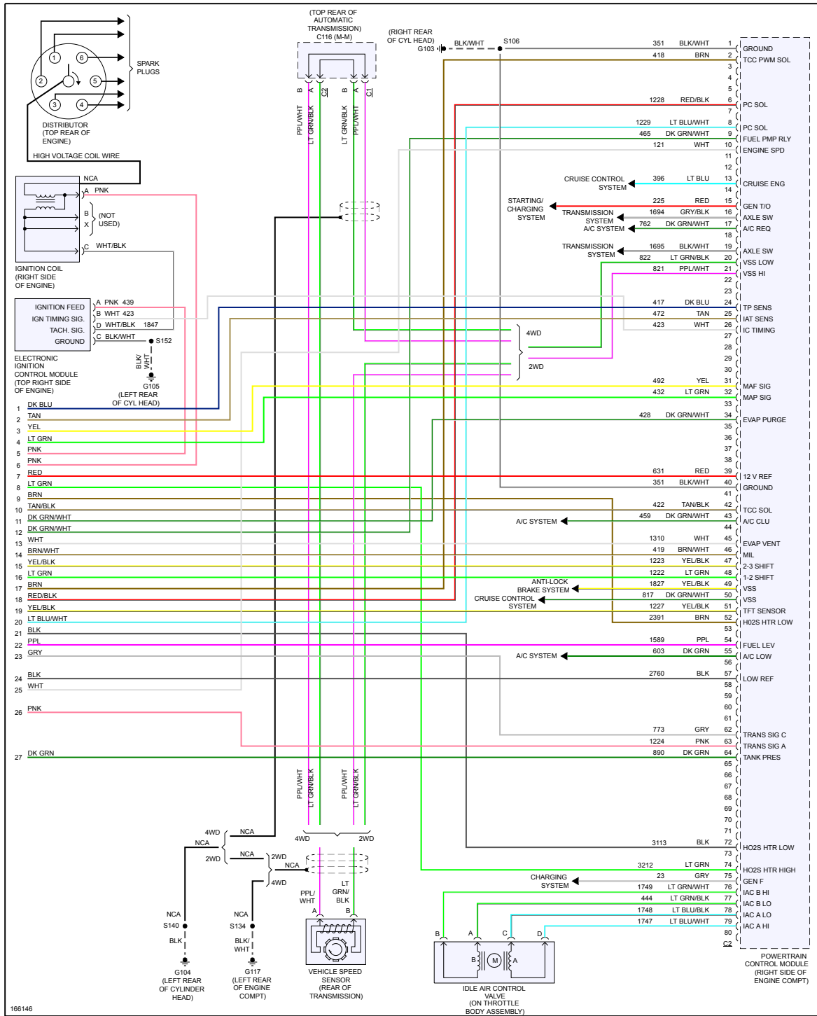
Fig 4: 4.3L VIN X, Engine Performance Circuit (4 of 4)
