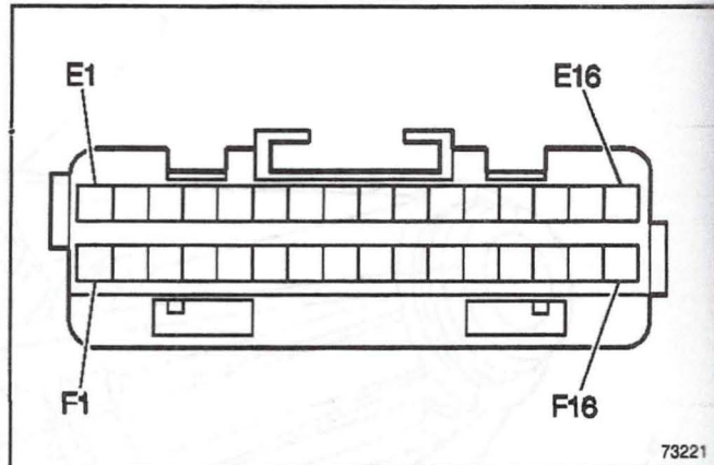
Transfer Case Shift Control Module Connector C1 (cont'd)
