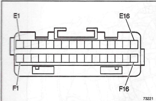
Transfer Case Shift Control Module Connector C1
