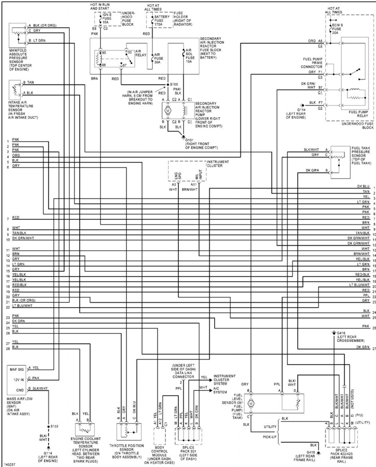
Fig. 16: 4.3L VIN W, Engine Performance Circuits (3 of 4)
