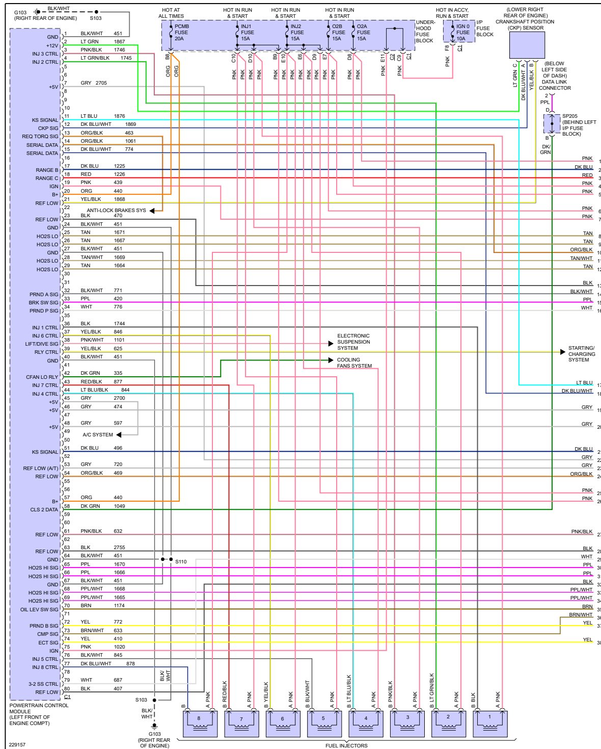
Fig 1: 5.3L VIN Z, Engine Performance Circuit (1 of 5)
