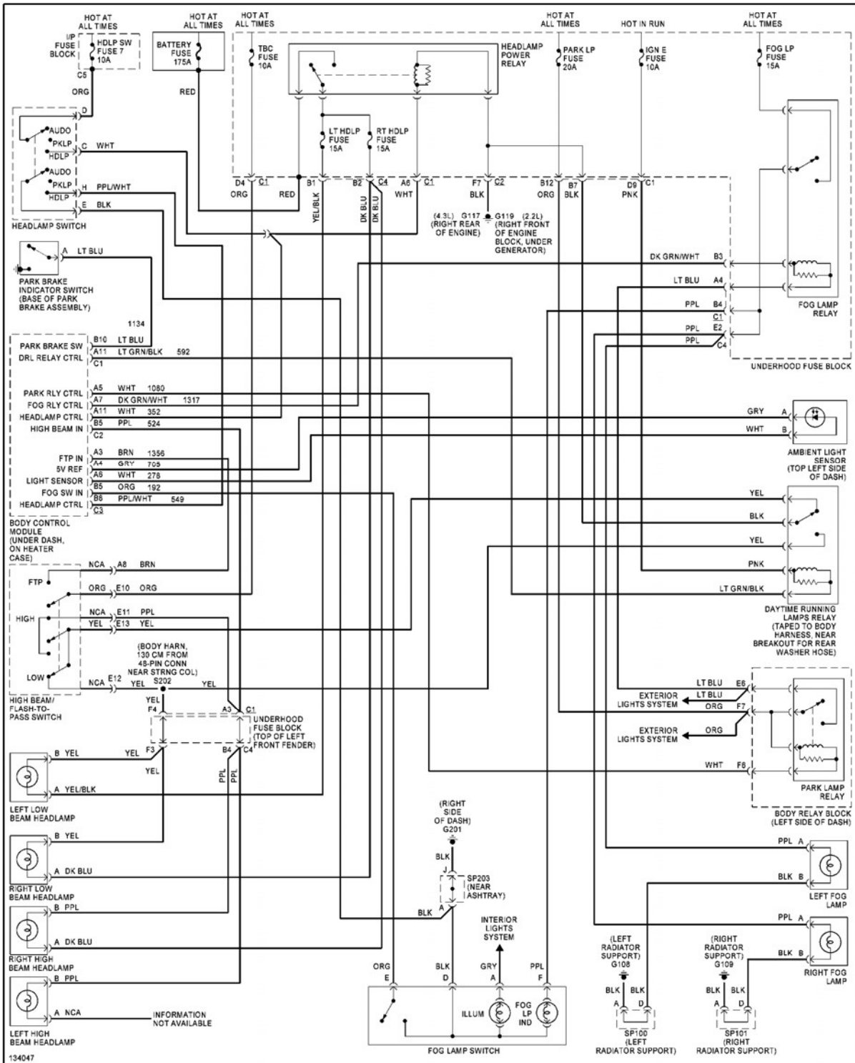
Fig. 23: Headlight Circuit, W/ ZR2
