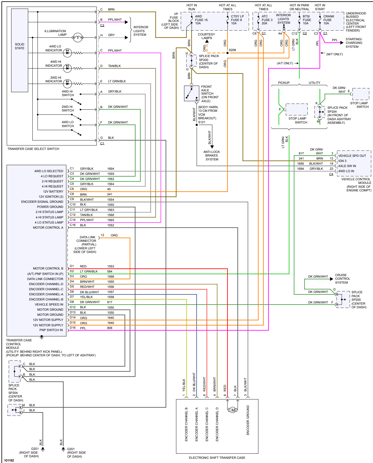
Fig 2: Electronic Transfer Case Circuit
