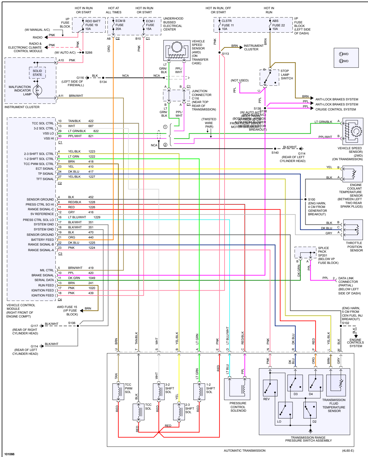
Fig 1: 4.3L (VIN W), Transmission Circuit, 4L60-E
