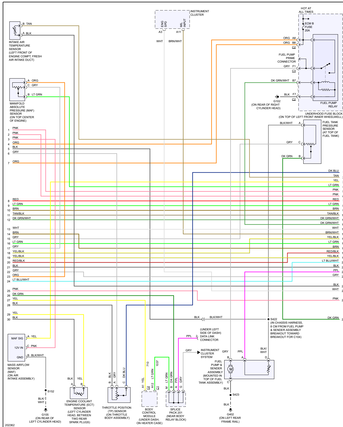
Fig 3: 4.3L VIN X, Engine Performance Circuit (3 of 4)
