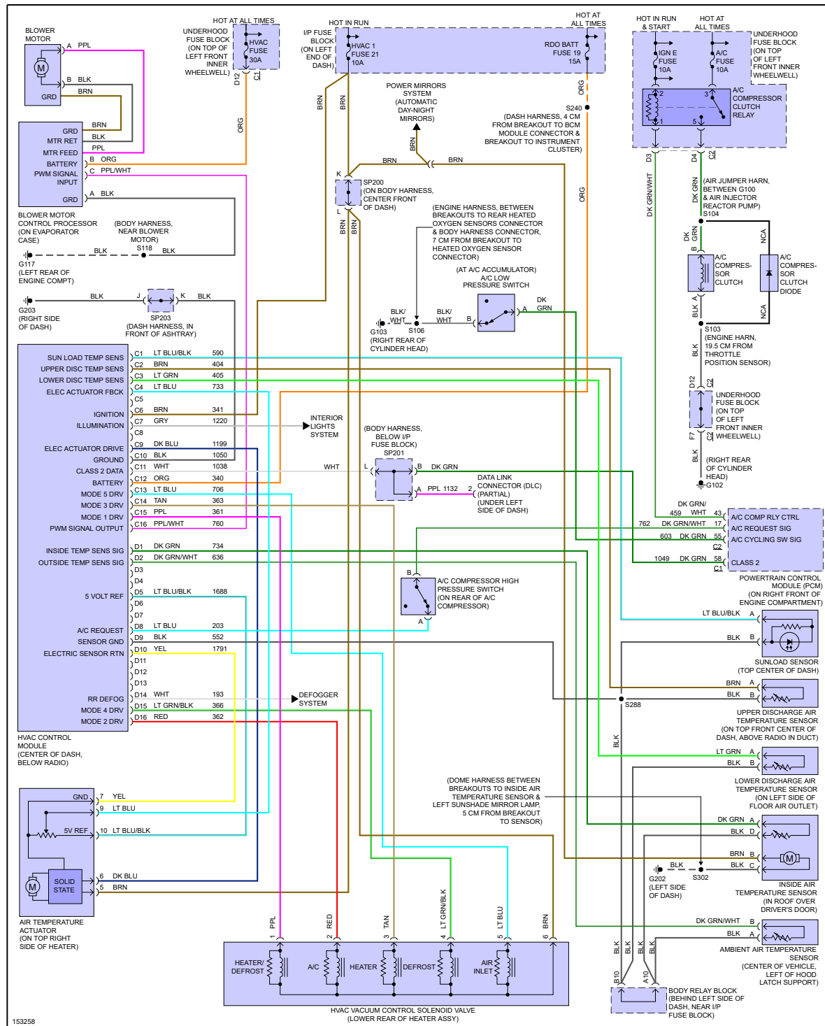
Fig 1: Automatic A/C Circuit
