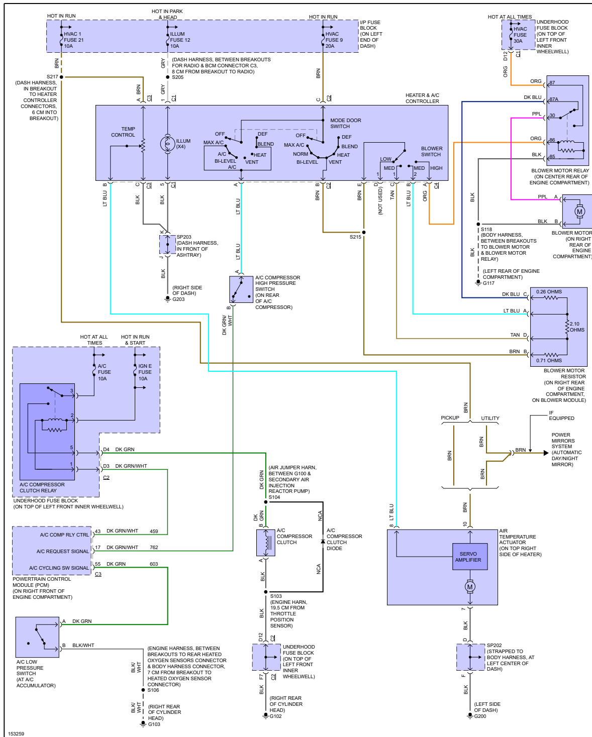
Fig 4: Manual A/C Circuit
