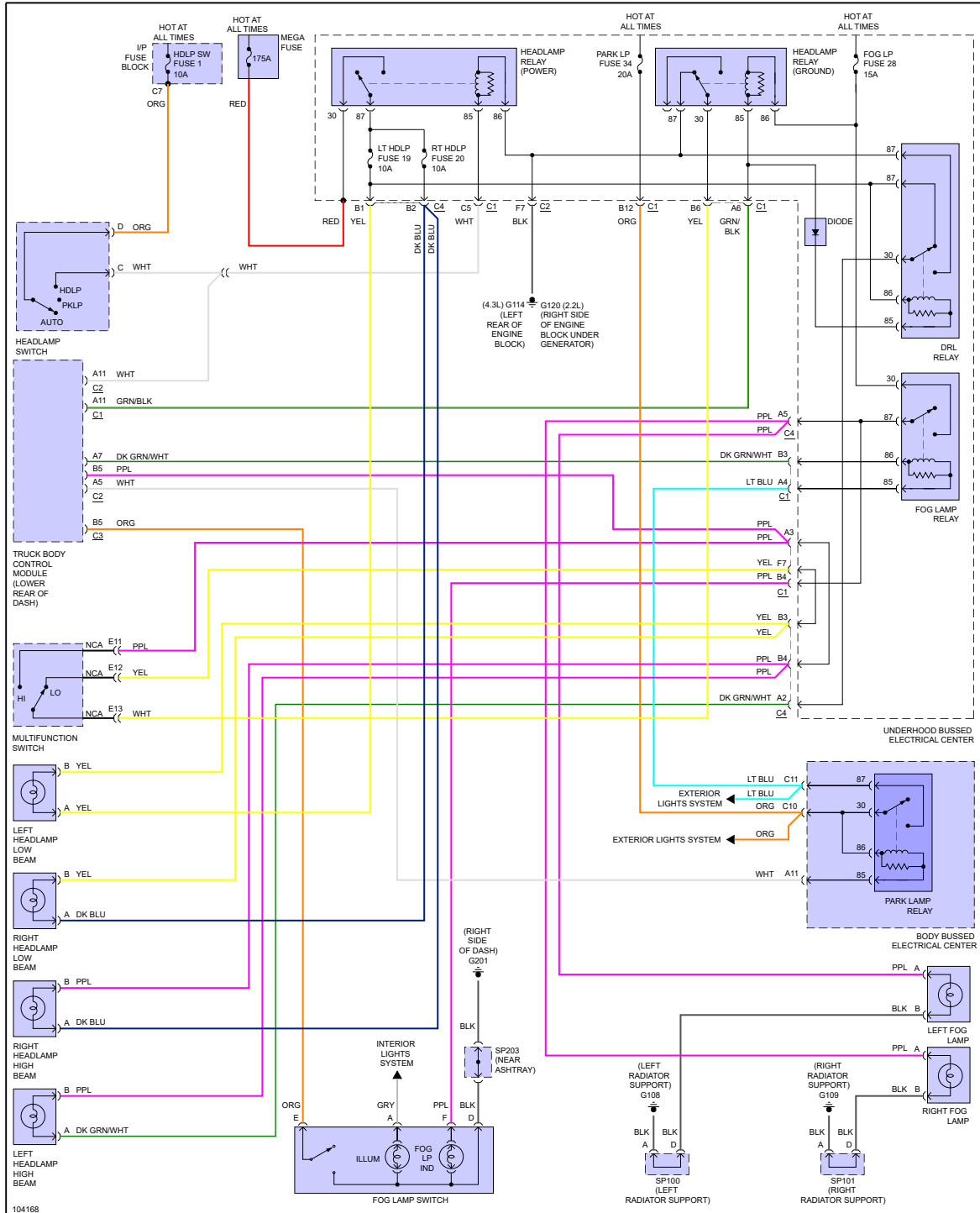
Fig 1: Headlamps & Fog Lamps Circuit
