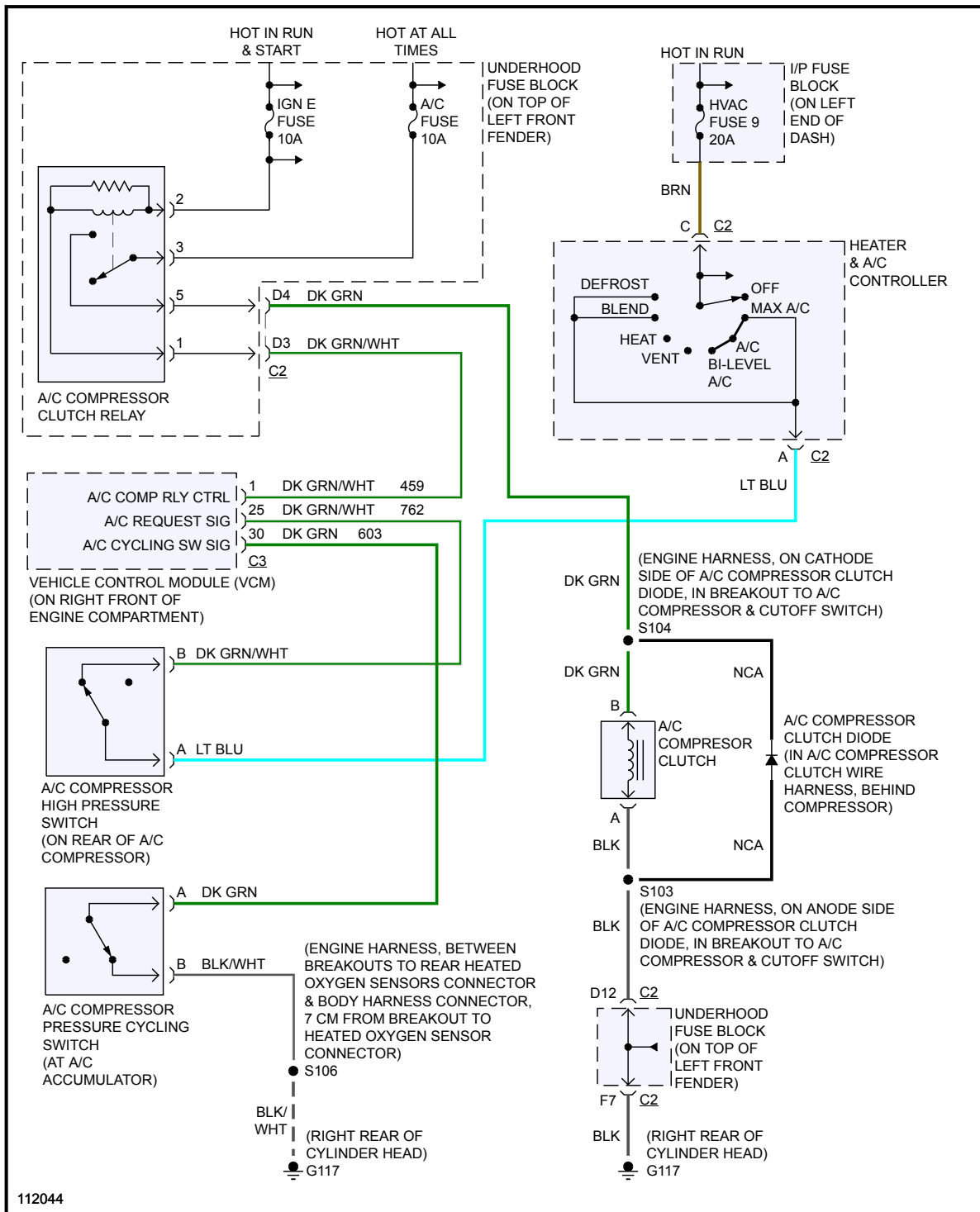
Fig 3: Compressor Circuit, Manual A/C
