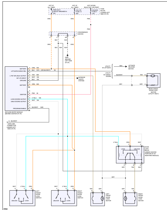
Fig 3: Keyless Entry Circuit, 2 Door
