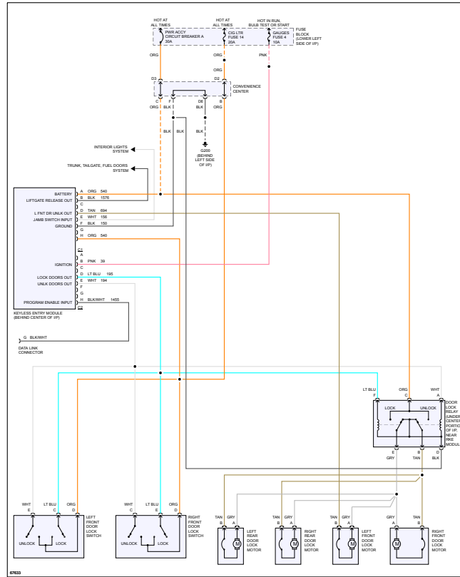
Fig 4: Keyless Entry Circuit, 4 Door
