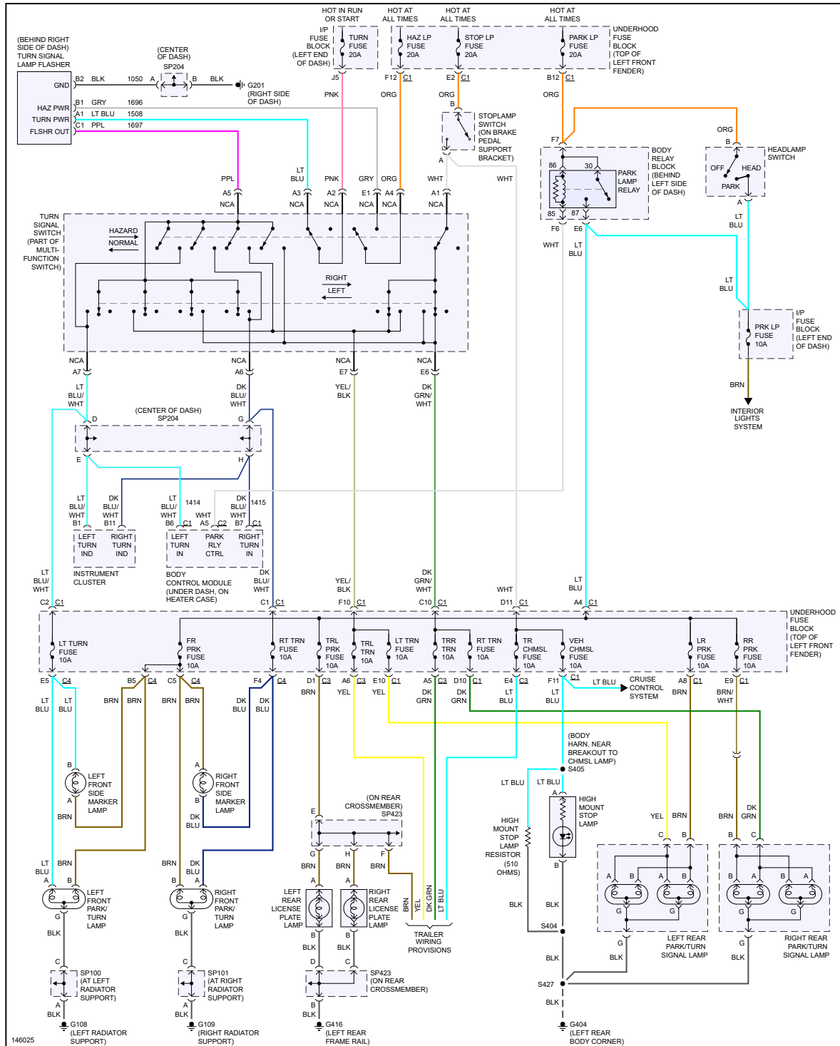
Fig 2: Exterior Lamps Circuit
