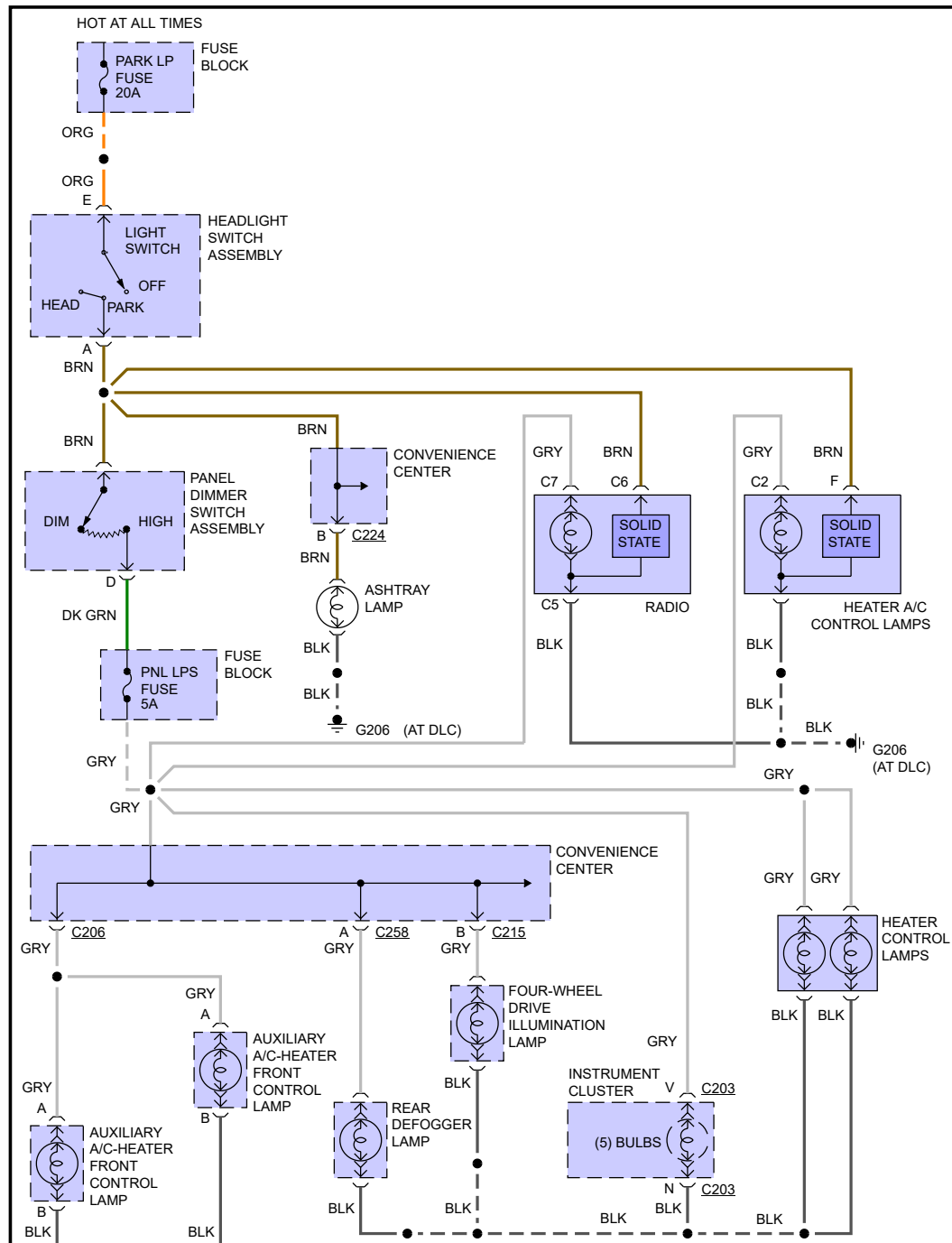
Fig 3: Instrument Illumination Circuit
