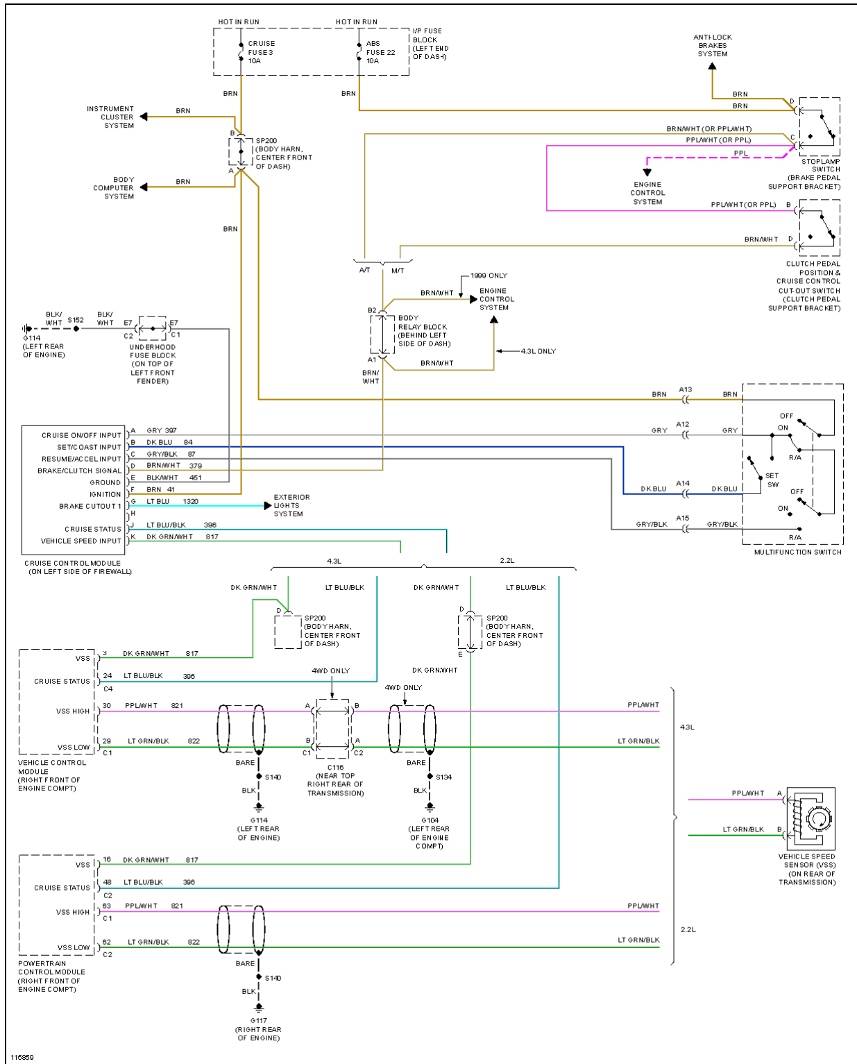
Fig. 15: Cruise Control Circuit
