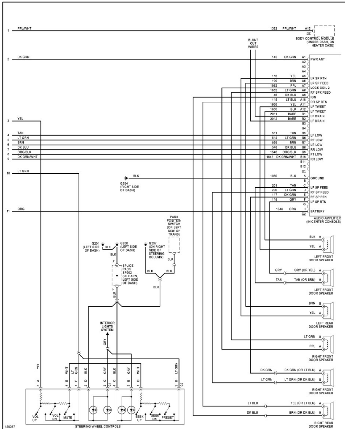
Fig. 48: Radio Circuits, W/ Amplifier (2 of 2)
